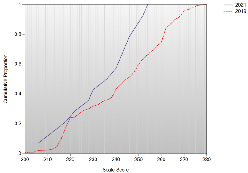
Cumulative Scale Score Distributions: Chemistry Grade 10
